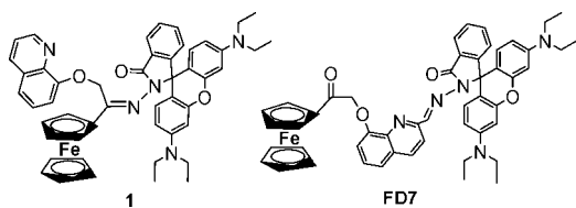
Figure 1. Chemical structures of 1 and FD7 .
