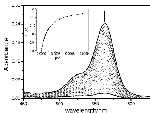
Figure 2. Changes in UV–vis absorption spectra of FD7 (20 \mu M) in ethanol/H 2 O (1:1, v/v, pH 7.4) solutions with various amounts of Cr 3+ ions (0–45 equiv). Inset: Absorbance at 565 nm of FD7 as a function of Cr 3+ concentration.
