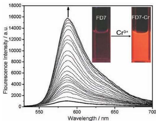
Figure 4. Fluorescence emission changes of FD7 (20 μM) in ethanol/H 2 O (1:1, v/v, pH 7.4) solutions upon addition of Cr 3+ (0–45 equiv). Each spectrum was acquired 1 min after Cr 3+ addition, \lambda_{\text{ex}} = 530 nm. Fluorescence photograph was obtained under irradiation of UV light (365 nm).
