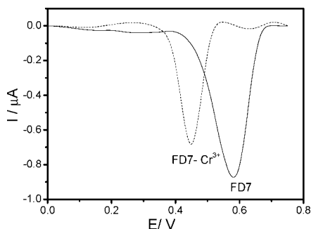
Figure 3. DPV of FD7 (100 μM) in ethanol solution in the absence and presence of 1.6 equiv of Cr 3+ with n -Bu 4 NPF 6 as supporting electrolyte.
