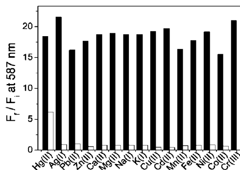
Figure 5. Fluorescence responses of FD7 (20 μM) to various metal ions (5 mM for Ca 2+ , Mg 2+ , Na + , K + , and Zn 2+ ; 900 μM for all other cations) in ethanol/H 2 O (1:1, v/v, pH 7.4). Bars represent the final integrated fluorescence response ( F_f ) over the initial integrated emission ( F_i ). White bars represent the addition of metal ions to a 20 μM solution of FD7 . Black bars represent the addition of Cr 3+ (45 equiv) to the solution. ( \lambda_{\text{ex}} = 530 nm).
