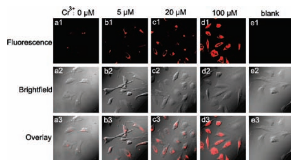
Figure 6. Confocal fluorescence, brightfield, and overlay images of HeLa cells. The cells were supplemented with 0\ \mu\text{M} (a1–a3), 5\ \mu\text{M} (b1–b3), 20\ \mu\text{M} (c1–c3), or 100\ \mu\text{M} (d1–d3) \text{CrCl}_3 in the growth media for 2.5 h at 37\ ^\circ\text{C} and then were stained with 20\ \mu\text{M} FD7 for 30 min at 37\ ^\circ\text{C} ( \lambda_{\text{ex}} = 543\ \text{nm} ). e1–e3 were reference cells without \text{Cr}^{3+} .
